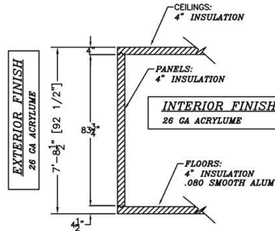
SECTION WALL WITH FLOOR
