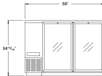
BBUC50-GD FRONT VIEW
