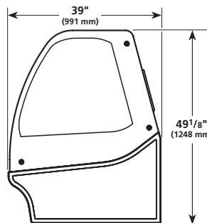
RIGHT VIEW
